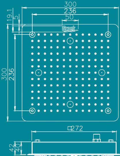
2D Drawing
