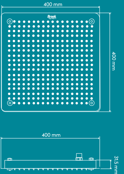
2D Drawing
