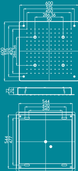
2D Drawing
