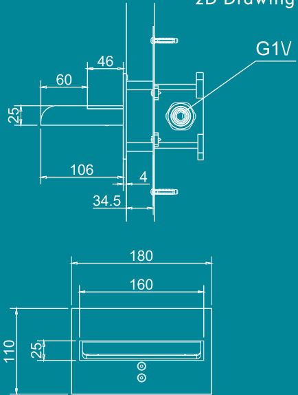
2D Drawing
