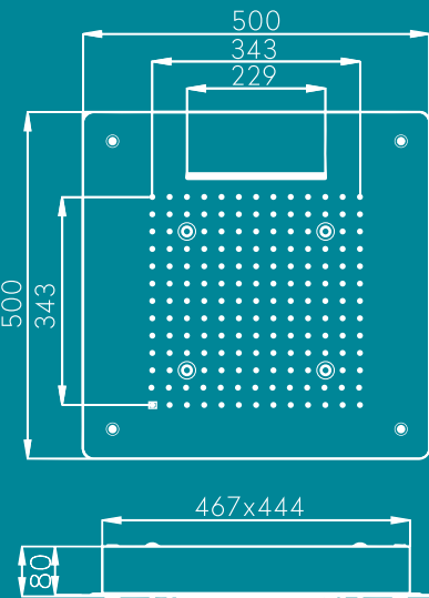
2D Drawing
