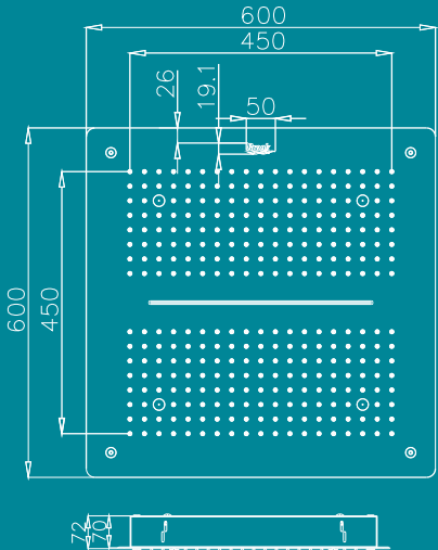
2D Drawing
