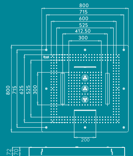
2D Drawing
