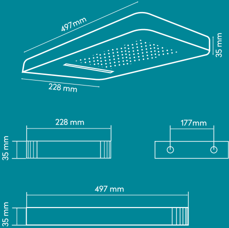
2D Drawing
