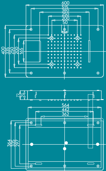
2D Drawing
