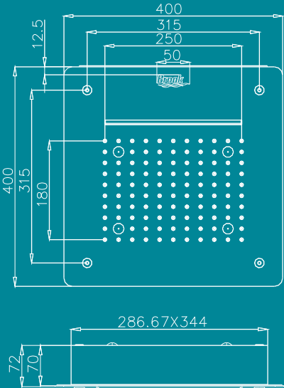
2D Drawing
